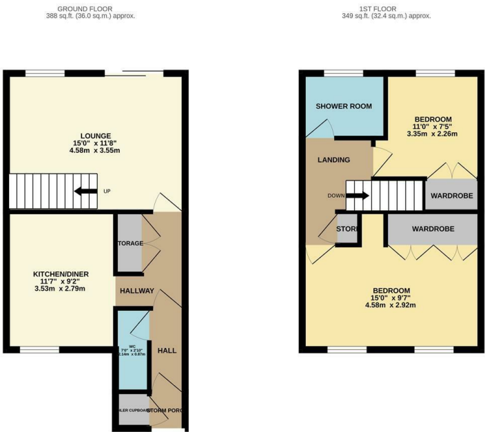
TOTAL FLOOR AREA: 737 sq.ft. (68.4 sq.m.) approx. Measurements are approximate. Not to scale. For illustrative purposes only. Made with Metreplus 12/2020
